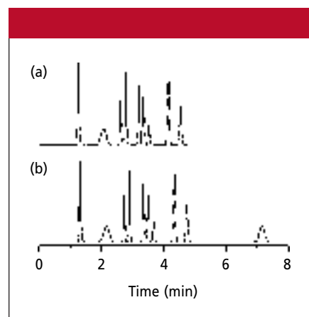
Figure 1: Simulated isocratic chromatograms for an eight-component mixture. Shown are (a) a normal 5-min run with an unexpected peak appearing at approximately 2 min and (b) the next injection with a 10-min run time.
